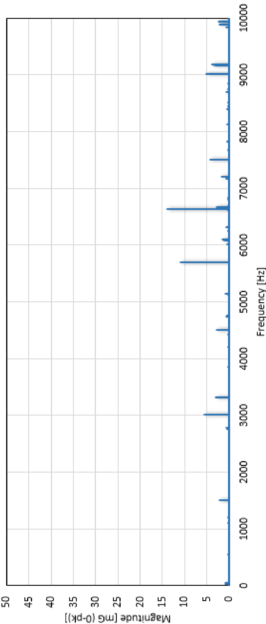
Typical vibration spectrum - nEXT85D/H ISO63 mounted on vibration isolator. Measured at pump inlet flange in axial direction.
